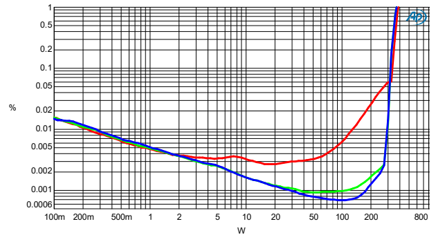
Figure 8: Ch2 THD+N vs. P_o @ 100Hz, 1kHz, 6.67kHz, R_L=8\Omega
