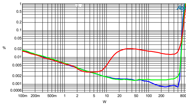
Figure 5: Ch1 THD+N vs. P_o @ 100Hz, 1kHz, 6.67kHz, R_L=4\Omega
