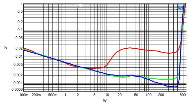
Figure 6: Ch2 THD+N vs. P_o @ 100Hz, 1kHz, 6.67kHz, R_L=4\Omega
