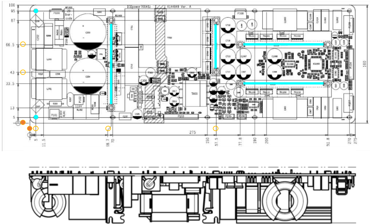
Figure 39: Mounting by top side Heat Sinks
