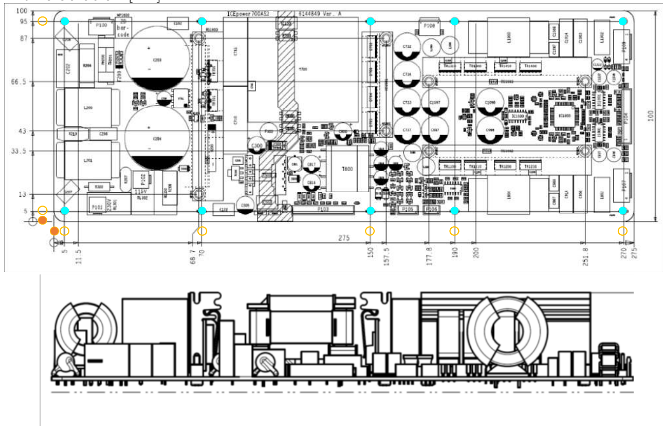
Figure 38: Mounting by bottom side spacers
