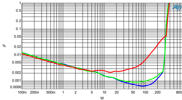
Figure 7: Ch1 THD+N vs. P_o @ 100Hz, 1kHz, 6.67kHz, R_L=8\Omega
