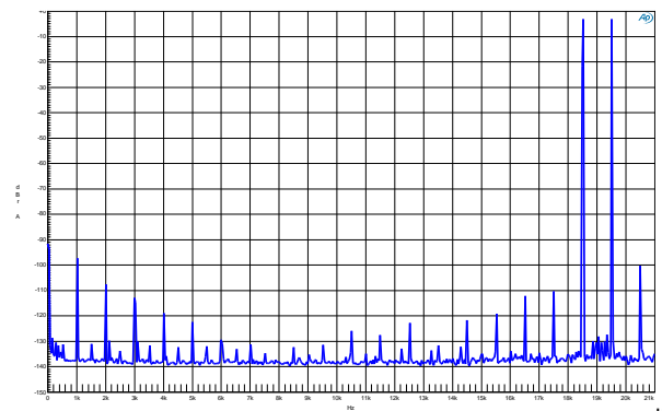
spectrum at 18.5kHz + 19.5kHz, PR/2 in 4Ω (blue).
