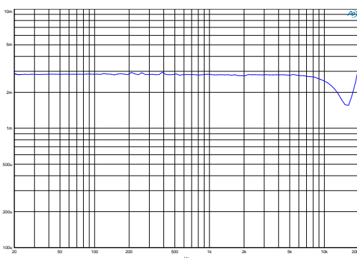
Output impedance
