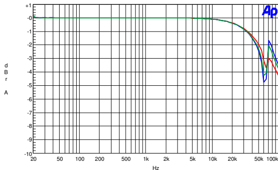
Frequency response into 8 (red), 4 (green) and 2 (blue) ohms
