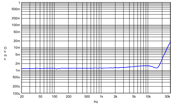
Output impedance, measured directly at J1
