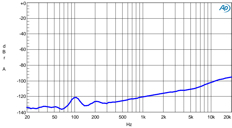
Figure 9: Channel separation 1200AS2, 20 Hz – 20 kHz @ P_o = 12\text{ W} / 4\ \Omega
