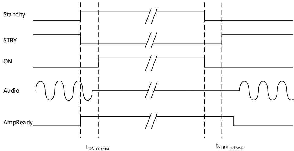
Figure 24: STBY and ON output timing
