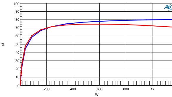
Figure 14: Power efficiency vs. output power, one channel driven, 230 V / 50 Hz (blue), 120 V / 60 Hz (red)
